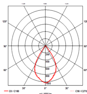
BONTEBOK 145 R 60°
