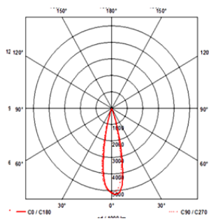
ETOSHA 130 R 30°
