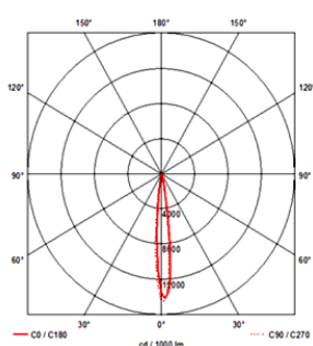
ETOSHA 130 R 20°
