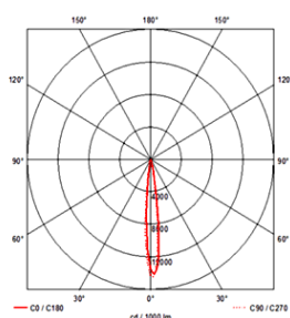
ETOSHA 170 R 20°
