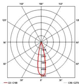
ETOSHA 170 R 30°
